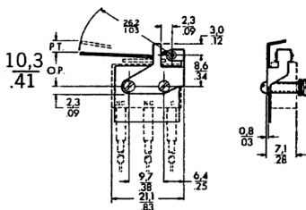
Figure 6. JS-307 Dimensions
